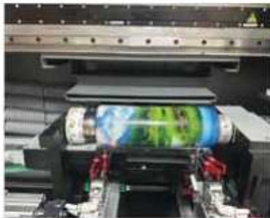
360° ROTARY UV
